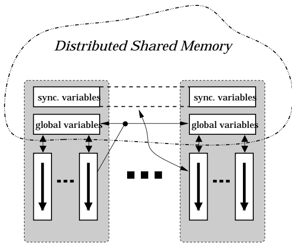
Figure 2. Multithreading and synchronization with Rthreads
