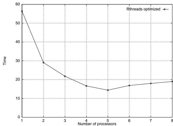
Figure 8. Performance evaluation of the distributed SOR algorithm for 2000 \times 500 matrices
