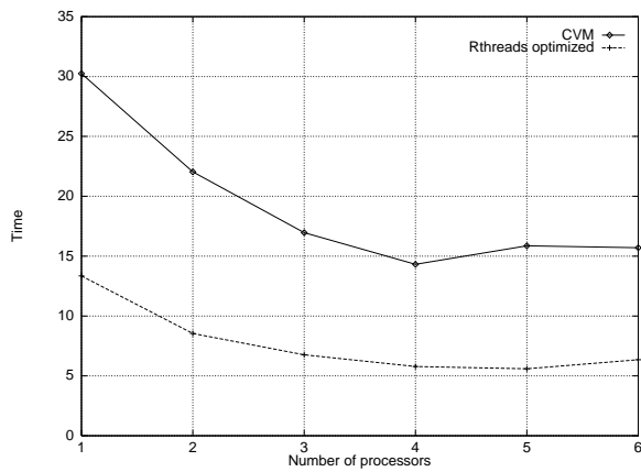
Figure 7. Performance evaluation of the distributed SOR algorithm for 600 \times 400 matrices
