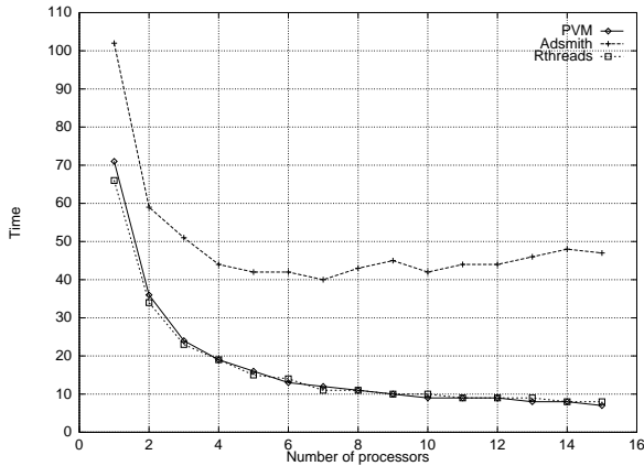
Figure 5. Performance evaluation of the distributed Mandelbrot calculation
