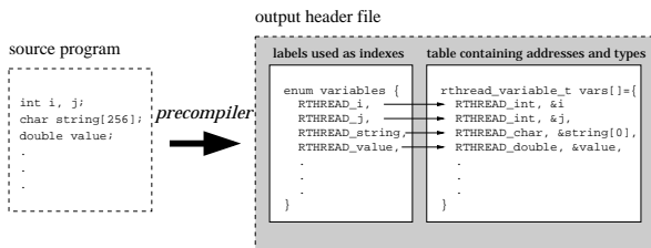
Figure 3. Identifiers generated by the precompiler
