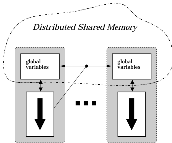
Figure 1. Distributed shared memory of Rthreads
