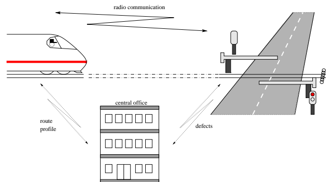
Fig. 4. Overview over the Radio-Based Crossing
