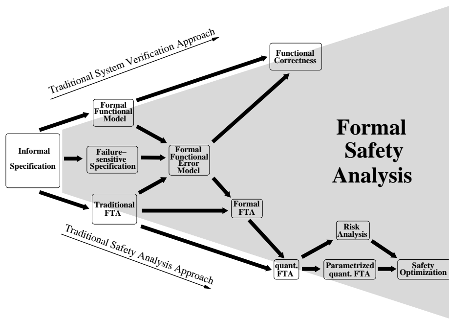
Fig. 1. Interaction of techniques
