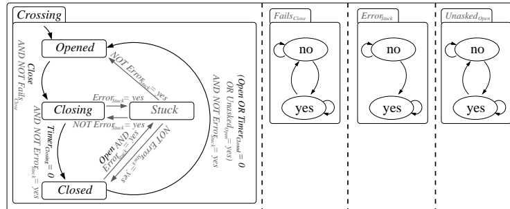
Fig. 6. Model of the crossing with failures
