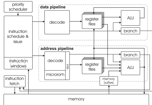
Figure 1. Block Diagram of CarCore.
