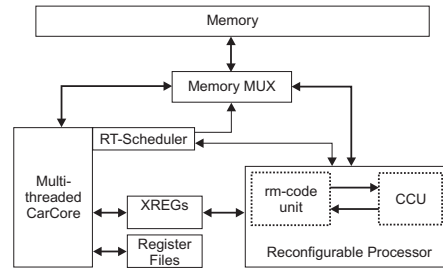
Figure 3. The CarCore reconfigurable unit
